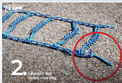
2. The outer fastening lock should face toward you.
